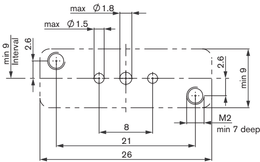
3/2 way connection
