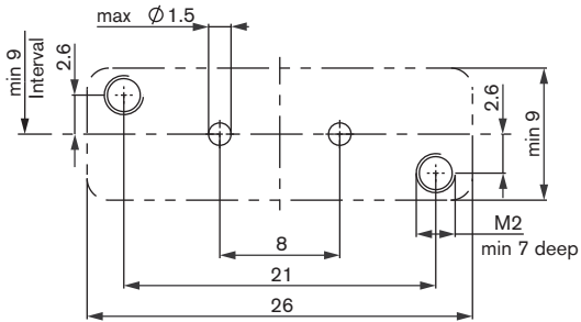
2/2 way connection
