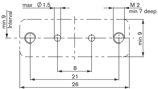
3/2 way connection
