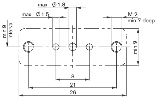
3/2 way connection
